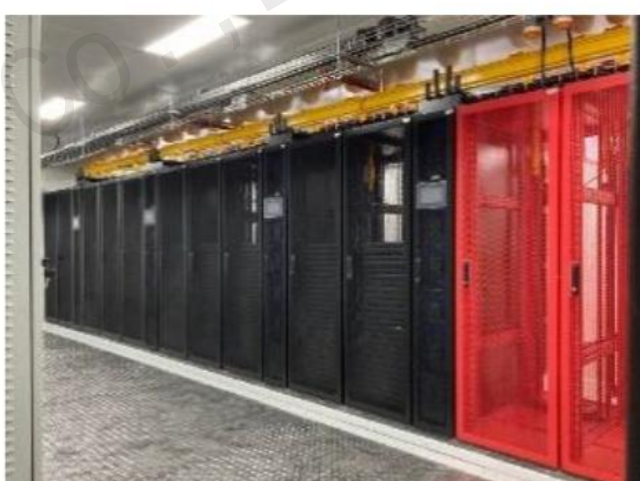
Inrow cooling solution
