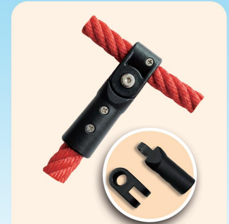
Item Code: SDN-NYL-003 Name: Nylon T-Connector Made of injection moulded PA Fix two sections of 16mm six strand steel wire rope Screw hole: 16mm
