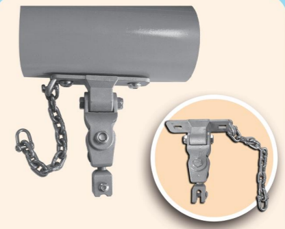
Item Code: SDN-SWI-003 Name: flower basket bolt Stainless steel swing hook, heavy duty Material: Stainless steel For commercial use swing set
