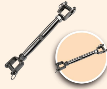
Item Code: SDN-STA-012 Name: Turnbuckle Material: Stainless Steel Application: Adjusting the tension - -of wire rope
