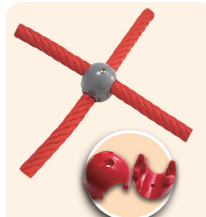
Item Code: SDN-NYL-004 Name: Nylon cross Connector(split type) For 16mm combination ropes Made of injection moulded PA (0.030kgs) It consisting of two parts are unre- -movable after assebly
