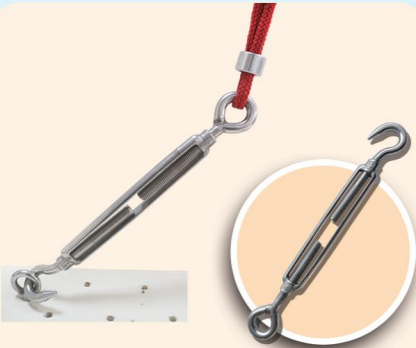
Item Code: SDN-STA-013 Name: flower basket bolt Turnbuckle M12*L31-44cm Made of stainless steel(0.414kgs)
