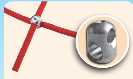
Item Code: SDN-ALU-001 Name: Aluminium X-connector For 16mm combination rope Made of aluminium To connect 2pcs ropes in a cross (0.052kgs)
