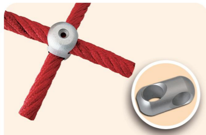
Item Code: SDN-ALU-008 Name: Aluminum Pipe Clamps (Surface oxidation process) Material: Aluminium Fix two sections of 16mm six strand- -steel wire rope Screw hole: 16mm
