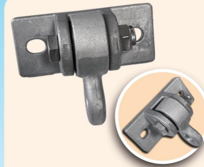
Item Code: SDN-SWI-001 Name: Swing Fixing Buckle Material: aluminum Specifications: 11*9cm Use: For securing swing ropes
