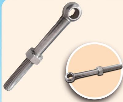
Item Code: SDN-STA-011 Name: Hinged Bolt Material: Stainless Steel Application: Connection of ends in - - wood or steel structures
