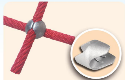
Item Code: SDN-ALU-004 Name: Aluminium Cross Connector For 12/14/16mm combination rope Made of aluminium (0.035kgs) To connect 2pcs ropes in a cross
