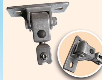
Item Code: SDN-SWI-002 Name: Swing Buckle Material: Stainless steel Specifications: 12*11cm Purpose: To secure swing ropes
