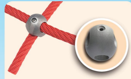
Item Code: SDN-ALU-003 Name: Solid Cross Connector(Big) For 16mm combination rope Made of casting aluminium (0.034kgs) To connect 2pcs ropes in a cross
