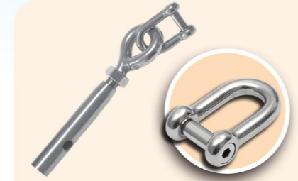
Item Code: SDN-STA-004 Name:Stainless steel D-shackle Made of 304 steel Size: M10 (0.106kgs)
