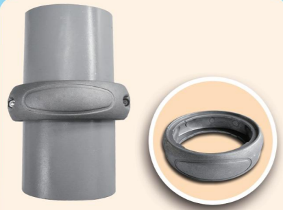
Item Code: SDN-ALU-044 Name:Hoop To connected 114mm steel post Made of Aluminium (0.287kgs) Need M8*30mm screws to fix
