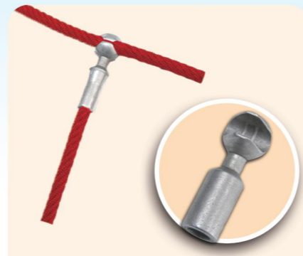
Item Code: SDN-ALU-013 Name: Aluminium T Connector Material: Aluminium Fix two sections of 16mm six strand- -steel wire rope Screw hole: 16mm
